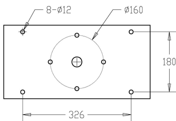
Monitor bottom mount hole
